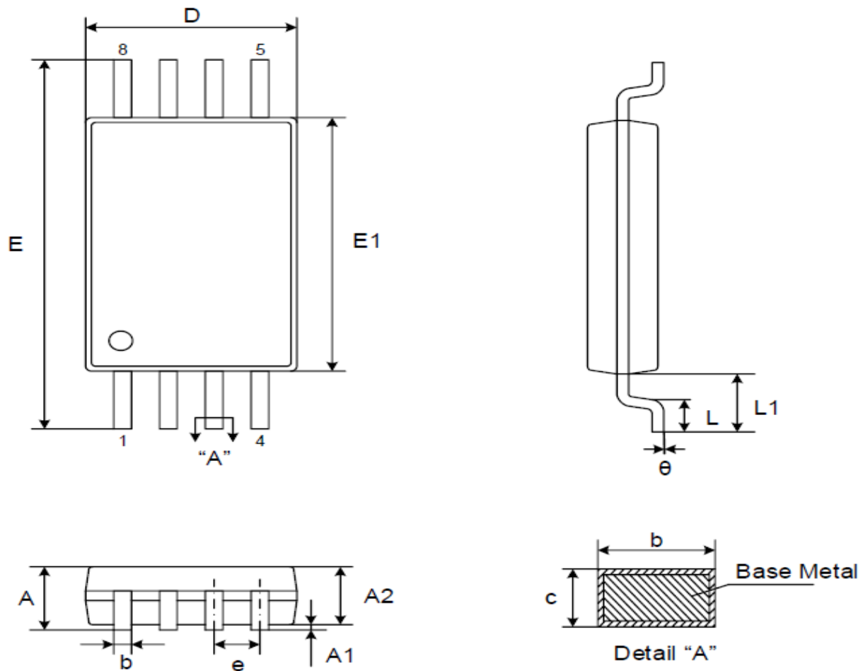
Figure 60 : TSSOP8(173mil) Package
