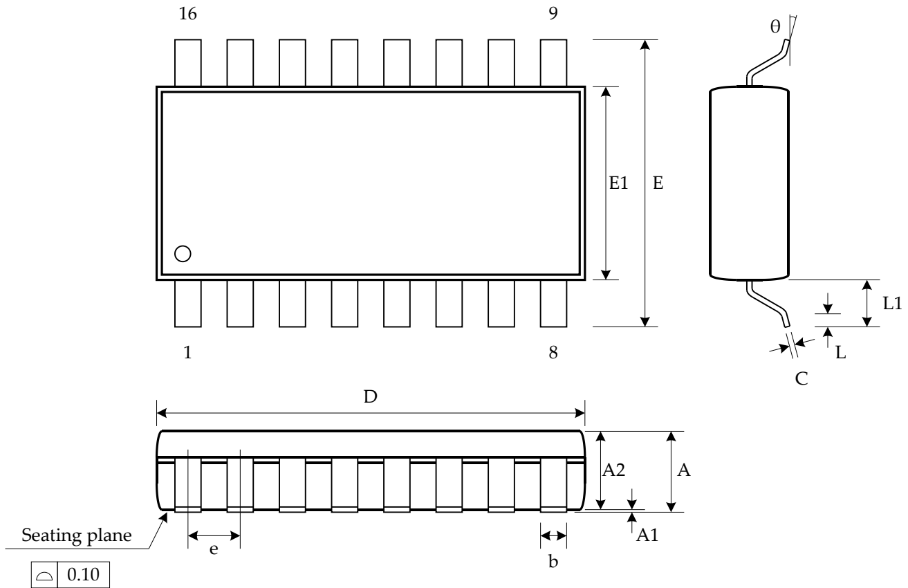
Figure 56: SOP16(300mil) Package
