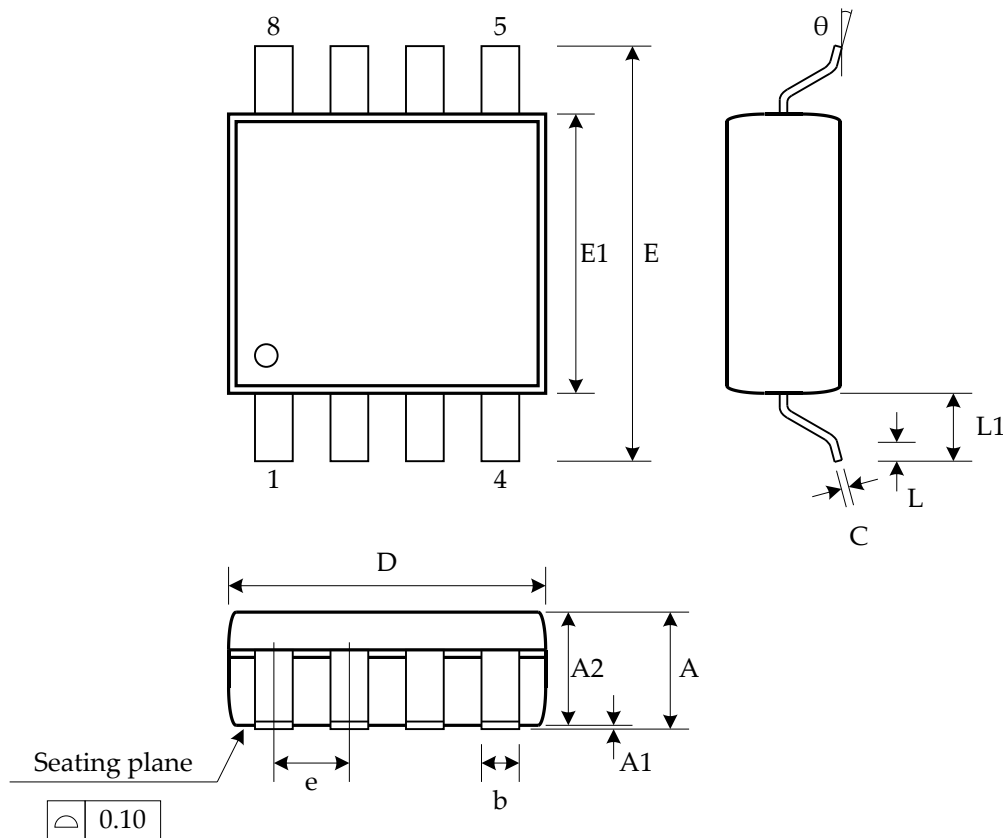
Figure 51: SOP8(208mil) Package
